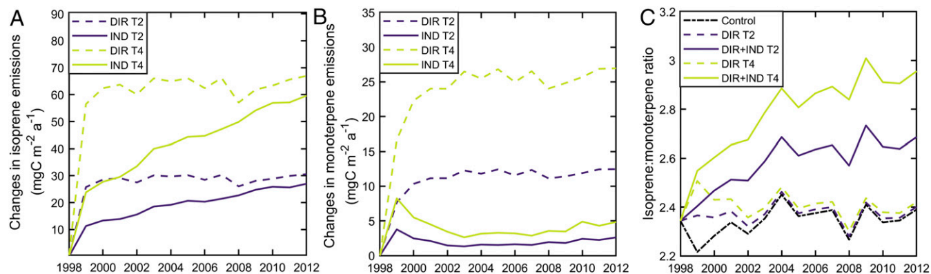
Fig. 3. Changes in modeled annual isoprene (A) and monoterpene (B) emissions due to direct and indirect effects, and the isoprene-to-monoterpene ratio for emissions (C) from each model simulation averaged over the Pan-Arctic land area. DIR were determined from the difference between the scenarios with 2 °C (DIR T2) or 4 °C (DIR T4) warming impacts on VOC production/emission and the control run. IND were determined from the difference between the simulations with both direct and indirect effects and those with only direct effects. Note the different y axis scales.
